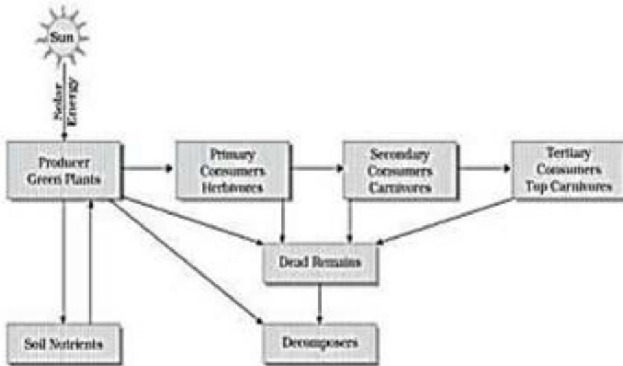
Figure 15.1 : Structure and functions of ecosystems
